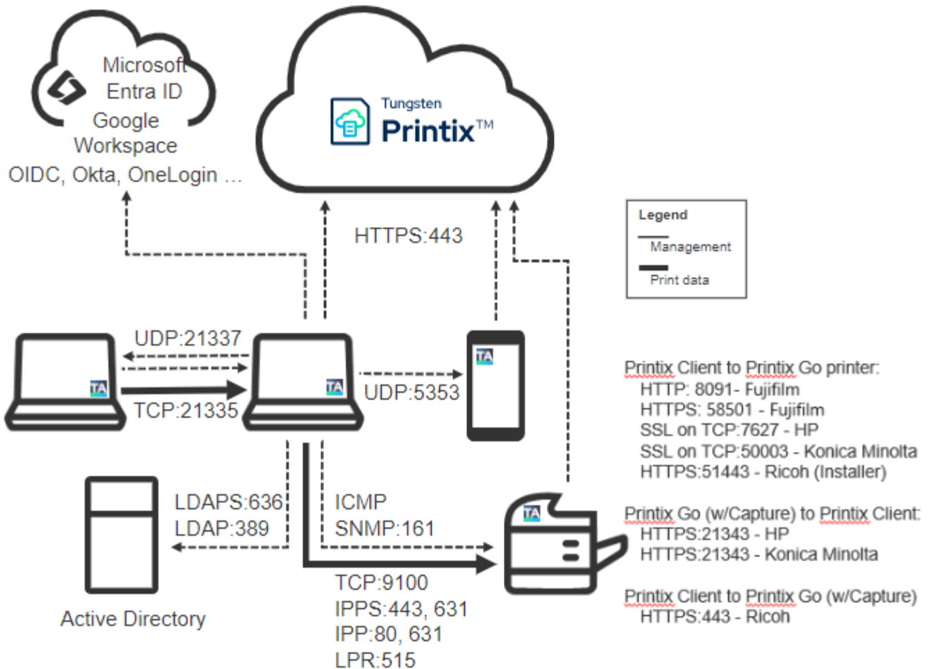
Overview over ports and network protocols used in Printix.
